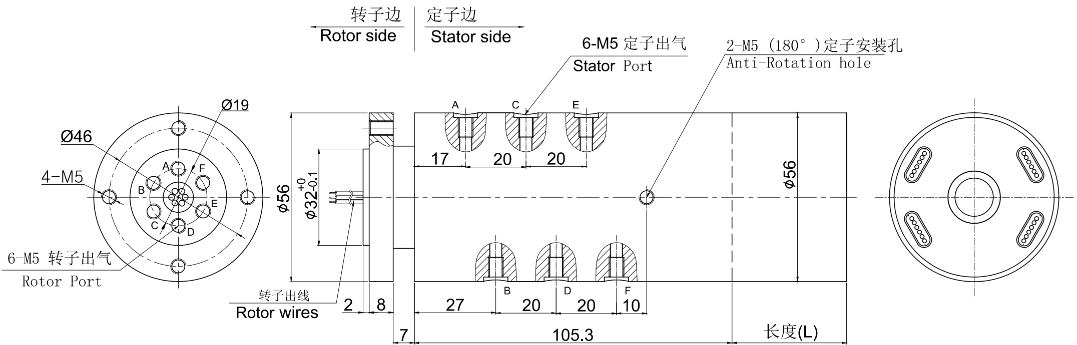
MAPH600-01+Electricity size
